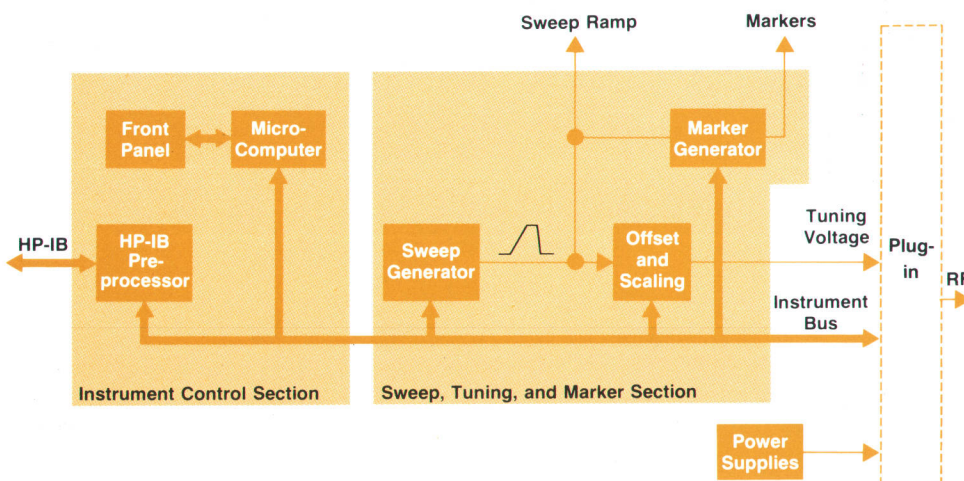
Fig. 7. Block diagram of the 8350A Sweep Oscillator.
