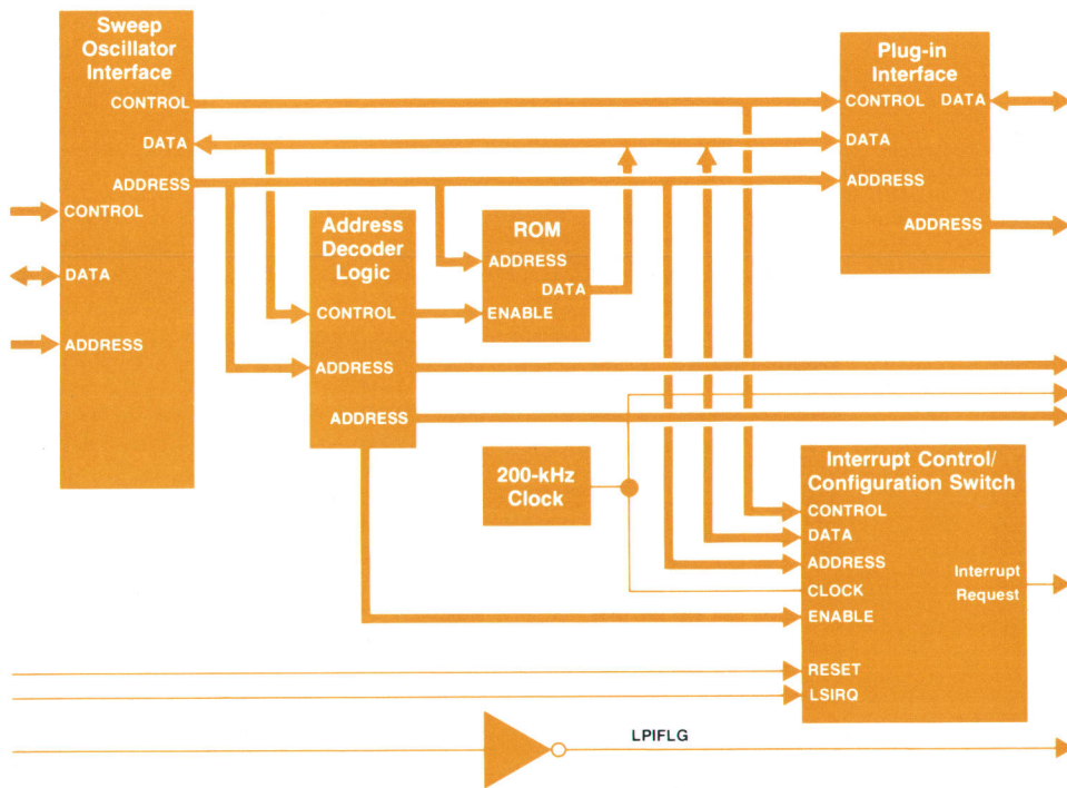
Fig. 6. Digital control section of the 83500 Series plug-ins.
