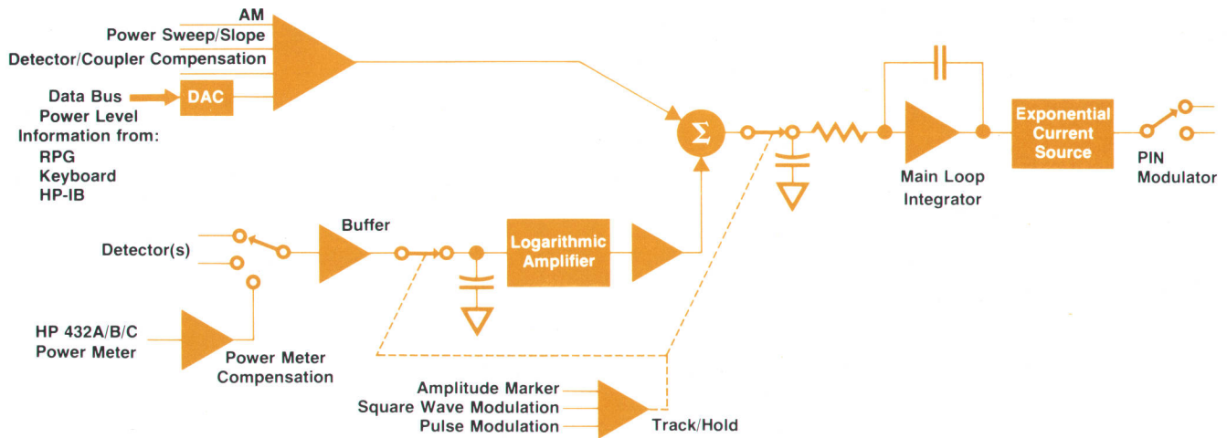
Fig. 10. Block diagram of the internal leveling circuits that maintain constant output power and provide for amplitude modulation.
