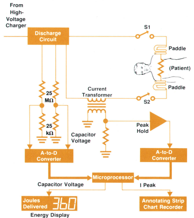
Fig. 7. Simplified block diagram of the 78660A's discharge control and recording circuitry.
