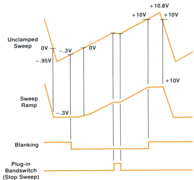
Fig. 9. Sweep waveforms generated by the circuit of Fig. 8.
