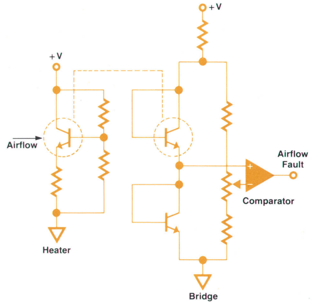
Fig. 12. Airflow sensor detects decreased airflow by sensing a temperature difference between a heated transistor and an unheated one.
