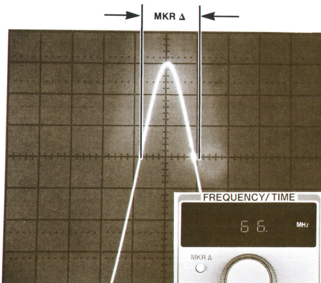
Fig. 4. Five independent, continuously variable markers identify significant frequencies. The marker difference function simplifies frequency bandwidth measurements as shown here. The frequency difference between any two of the five markers is displayed.
