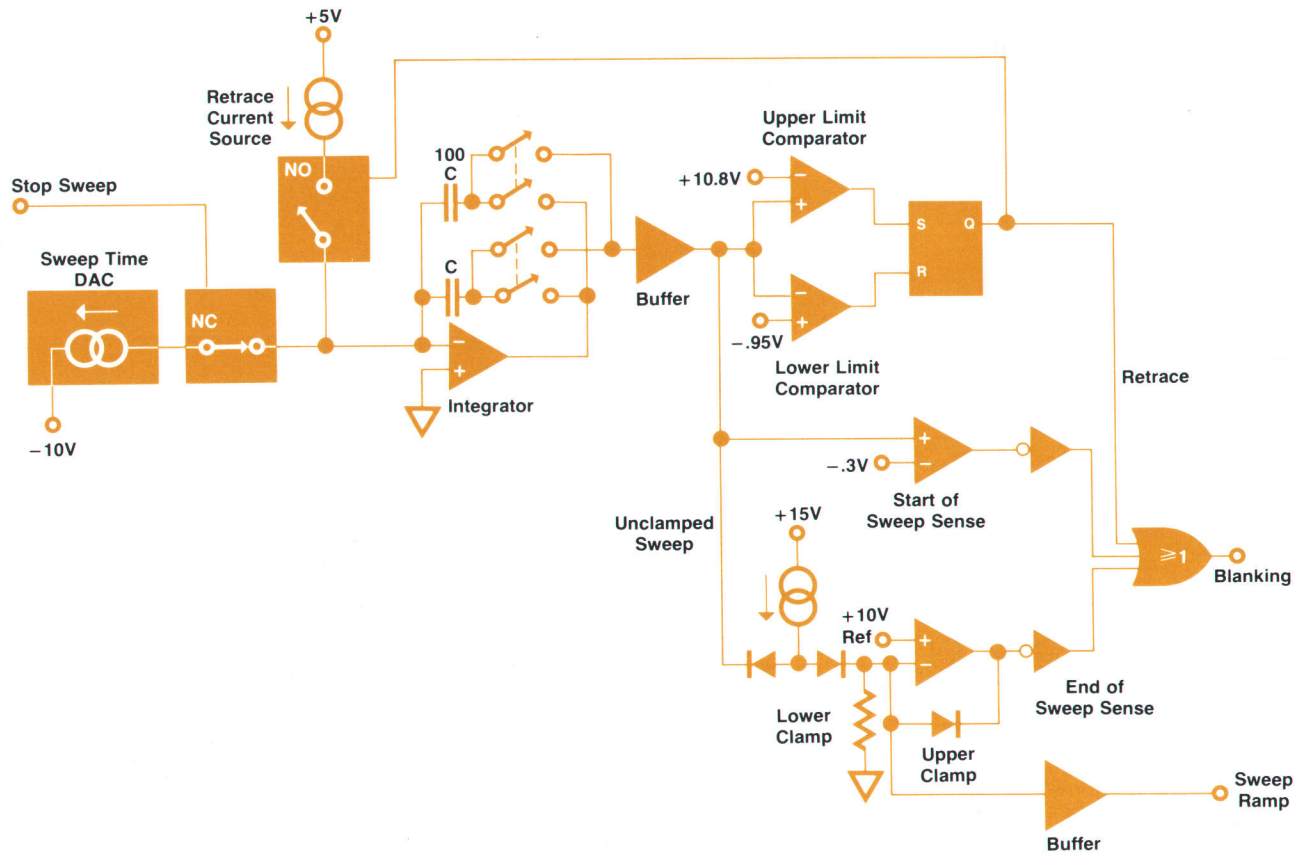
Fig. 8. 8350A sweep generation circuits.
