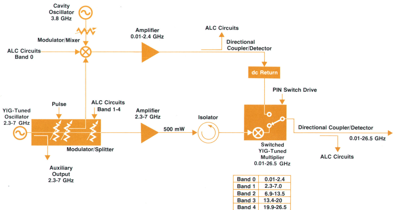
Fig. 5. Block diagram of the 83595A 0.01-to-26.5-GHz plug-in. The 83594A 2-to-26.5-GHz plug-in is made by deleting the low-frequency section. The 83592A (0.01-20 GHz) and the 83590A (2-20 GHz) are similar, but use RF components designed to operate to only 20 GHz.
