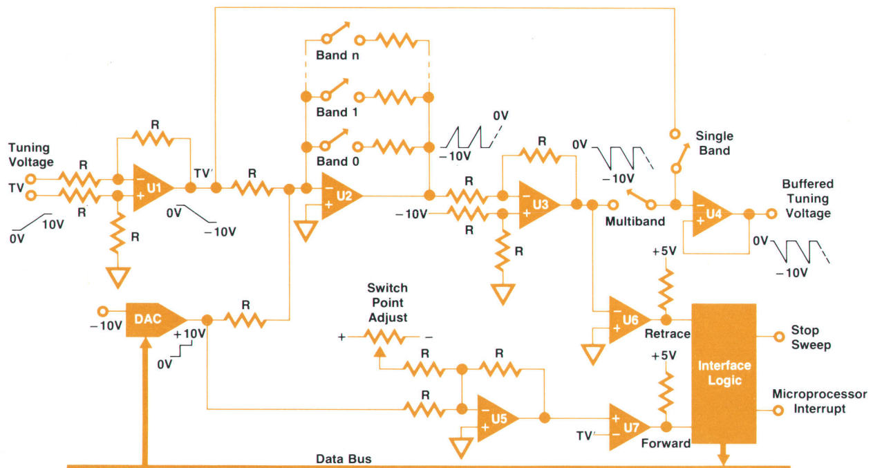
Fig. 8. Plug-ins capable of very wide sweeps actually sweep several individual frequency bands in sequence. The additional circuitry required to do this is shown here.
